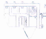
Model 126S Sheeting Clamp Clamp force 1112 kN Weight 991 kg
