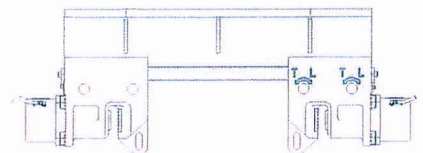
Model 80S Casing Clamps w/ 5' Beam Clamp force 1423 kN Weight 1279 kg
